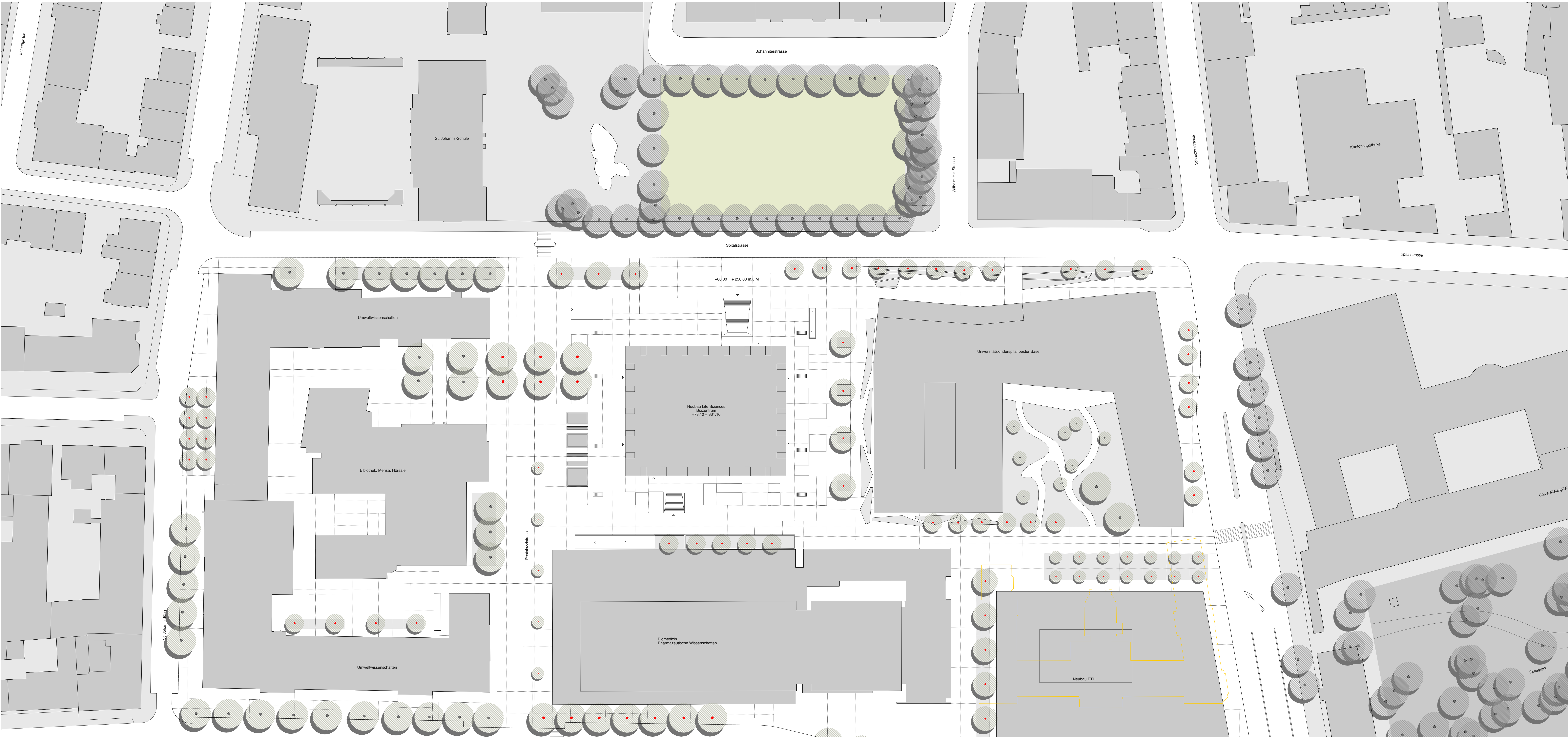
Situation 1:500
